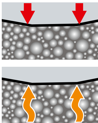
Irregular shaped and sized cells reduce the resistance to indentation
