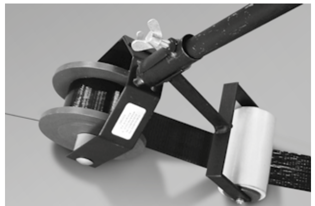
Single-side tape reel - H367 0003
